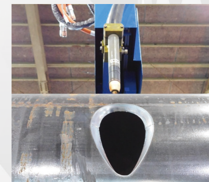
Tear drop hole with bevel
