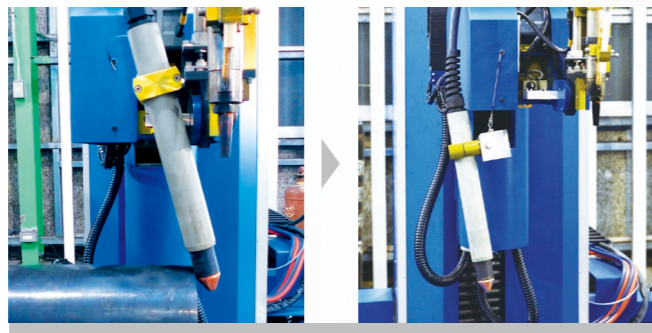
Magnetic torch protection [ Break-away torch system ]
